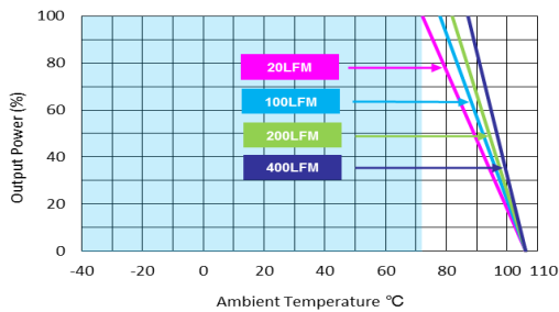
MJWI15-24S033, MJWI15-48S033 Derating Curve without Heatsink
