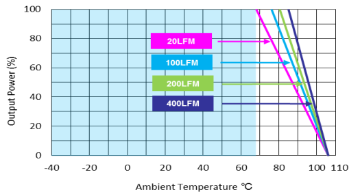
MJWI15-24S05, MJWI15-24S12, MJWI15-48S05 Derating Curve without Heatsink
