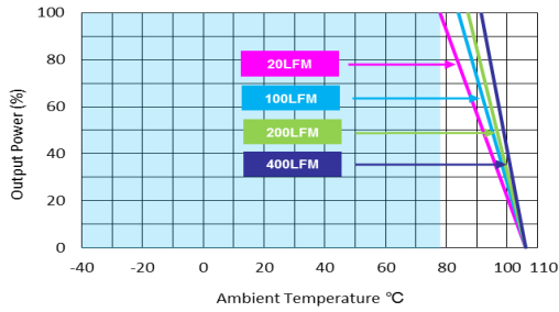
MJWI15-24S24, MJWI15-48S24 Derating Curve without Heatsink
